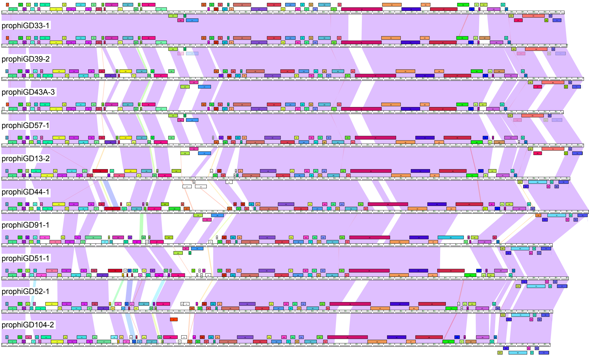
Figure S10. Genome comparisons of ClusterMabC. See Figure S3 for details.
