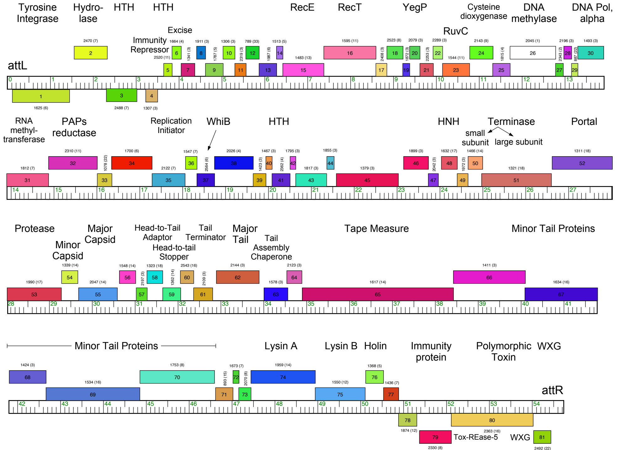
Figure S16. Genome organization of prophiGD11-3, Cluster MabF. See Figure S2 for details.
