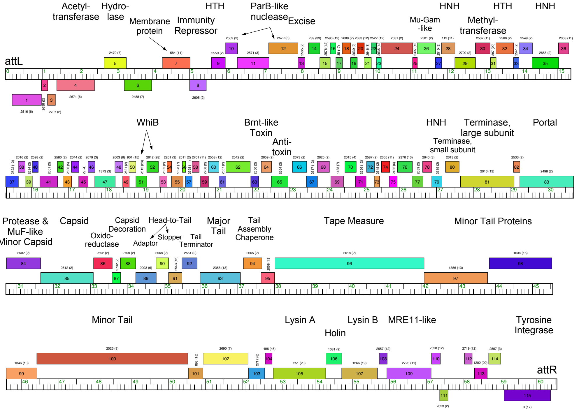
Figure S4. Genome organization of prophage GD02-2, Cluster MabA2. See Figure S2 for details.
