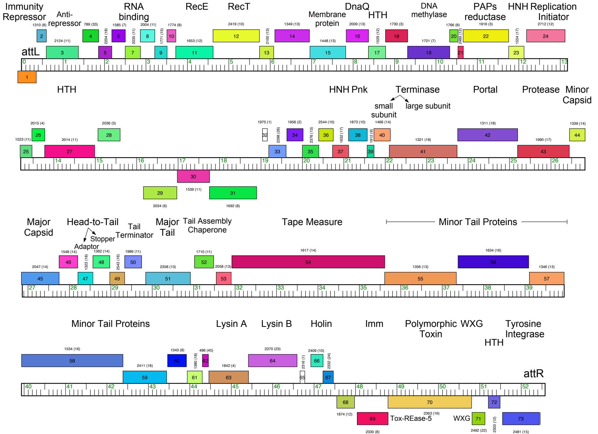
Figure S9. Genome organization of prophage GD57-1, Cluster MabC. See Figure S2 for details.
