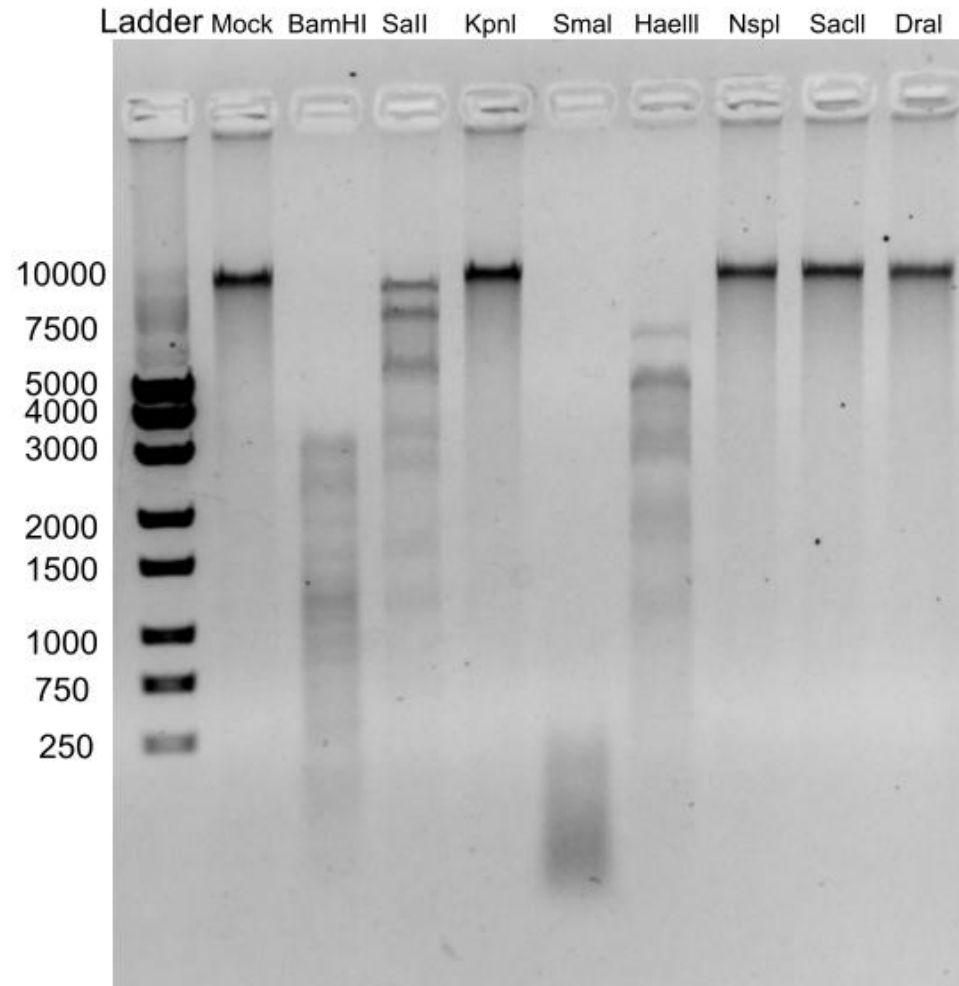
Restriction enzyme digest of the Azhaar genome. 800ng of purified Azhaar genomic DNA was digested with indicated enzymes for 1 hour at 37 degrees celsius, run on a 1% agarose gel containing 10ug/ml ethidium bromide, and imaged.
