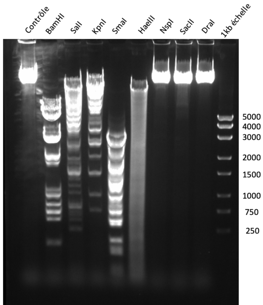
Restriction enzyme digest of Episkey's genome. 1 \mu g of purified Episkey genomic DNA was ingested with the indicated enzymes for 80min at 37°C, run on 1% agarose gel containing TAE and imaged on the Bio-rad imager using the ethidium bromide.
