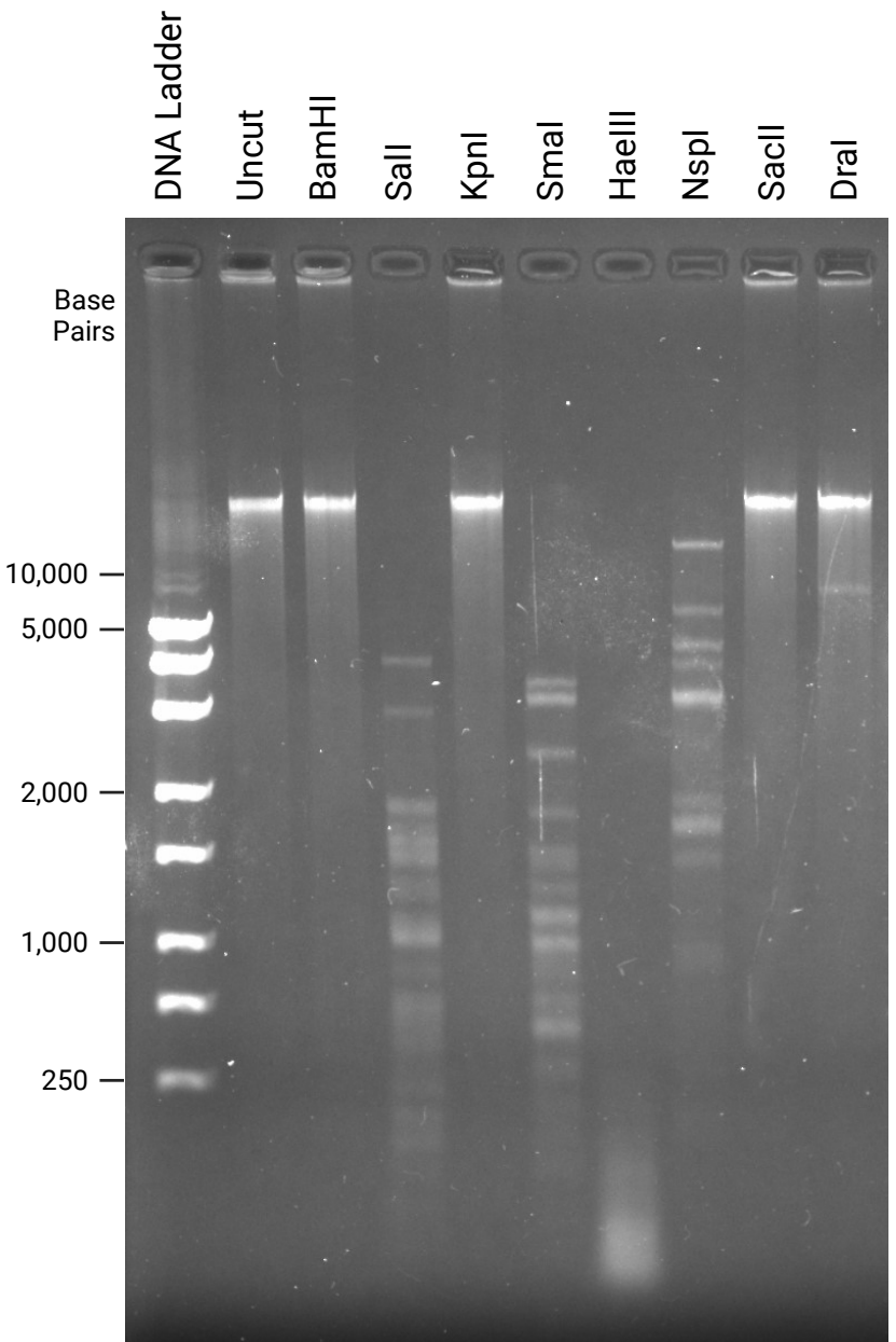
Figure 3. Restriction enzyme digest of Henderson genome. Purified Henderson genomic DNA was digested with the indicated enzymes for 1 hr at 37°C, run on a 1% agarose gel containing ethidium bromide, and imaged. Figure created with BioRender.com.
