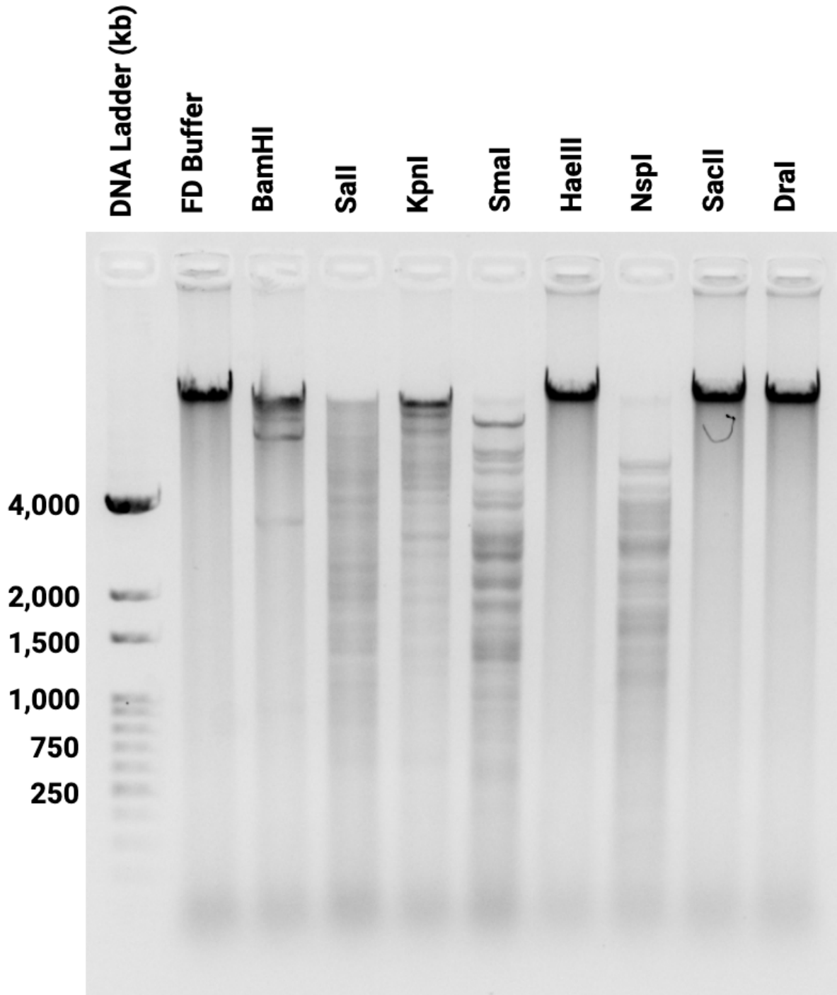
Restriction enzyme digest of Jask genome. Purified Jask genomic DNA was digested with indicated enzymes for 1 hr at 37°C, run on a 1% agarose gel containing 10ug/mL ethidium bromide, and imaged.
