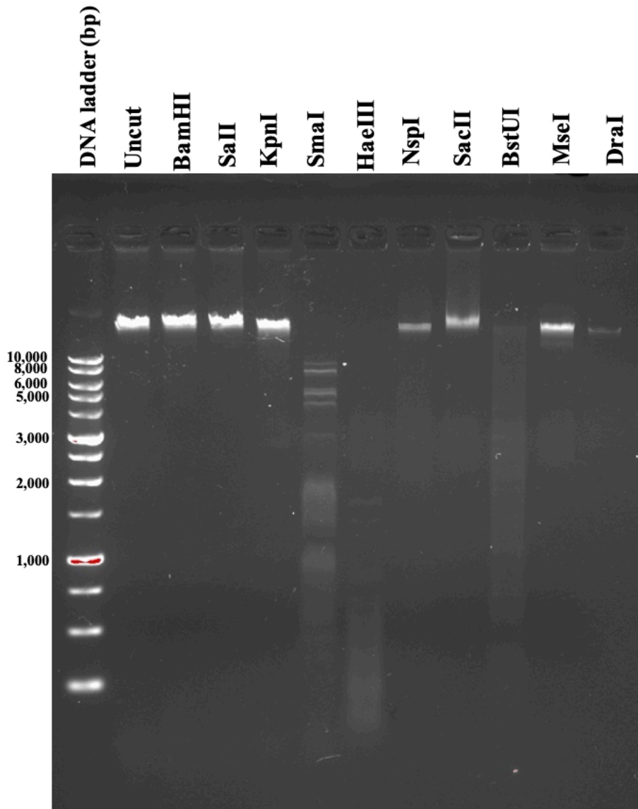
Restriction digest image of LilBoggy genome. 2 mL of purified LilBoggy genomic DNA was digested with the indicated enzymes for 1 hr at 37°C, run on a 1% agarose gel containing 10 mg/ml ethidium bromide.
