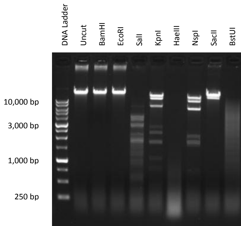
Restriction enzyme digest of SideCharacter genome. 1 \mu\text{g} of purified SideCharacter genomic DNA was digested with the indicated enzymes for 30 min at 37°C, then run on a 1% agarose gel containing 0.5 \mu\text{g}/\text{ml} ethidium bromide.
