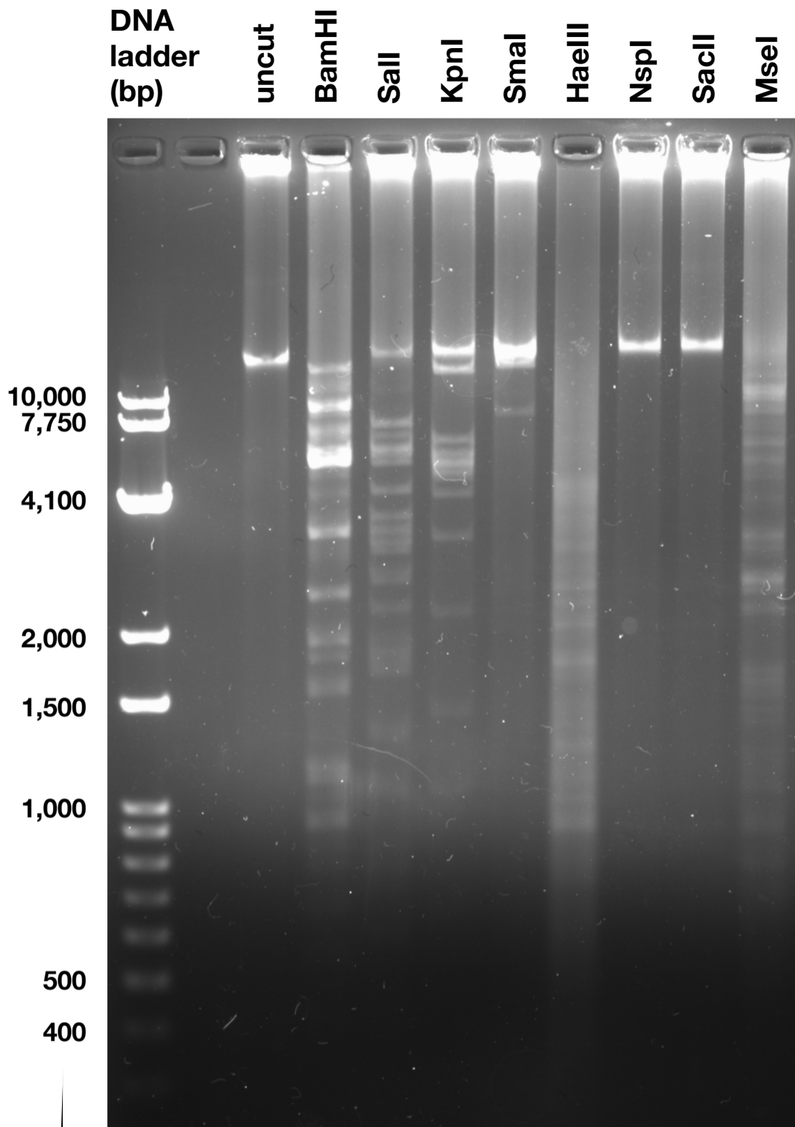
Restriction enzyme digest of the Soypaloi genome. 500ng of purified Soypaloi genomic DNA was digested with the indicated enzymes for 1 hr at 37°C, run on a 1% agarose gel containing 10 µg/ml ethidium bromide, and imaged. DNA ladder is in-house prepared PSU 100bp ladder.
