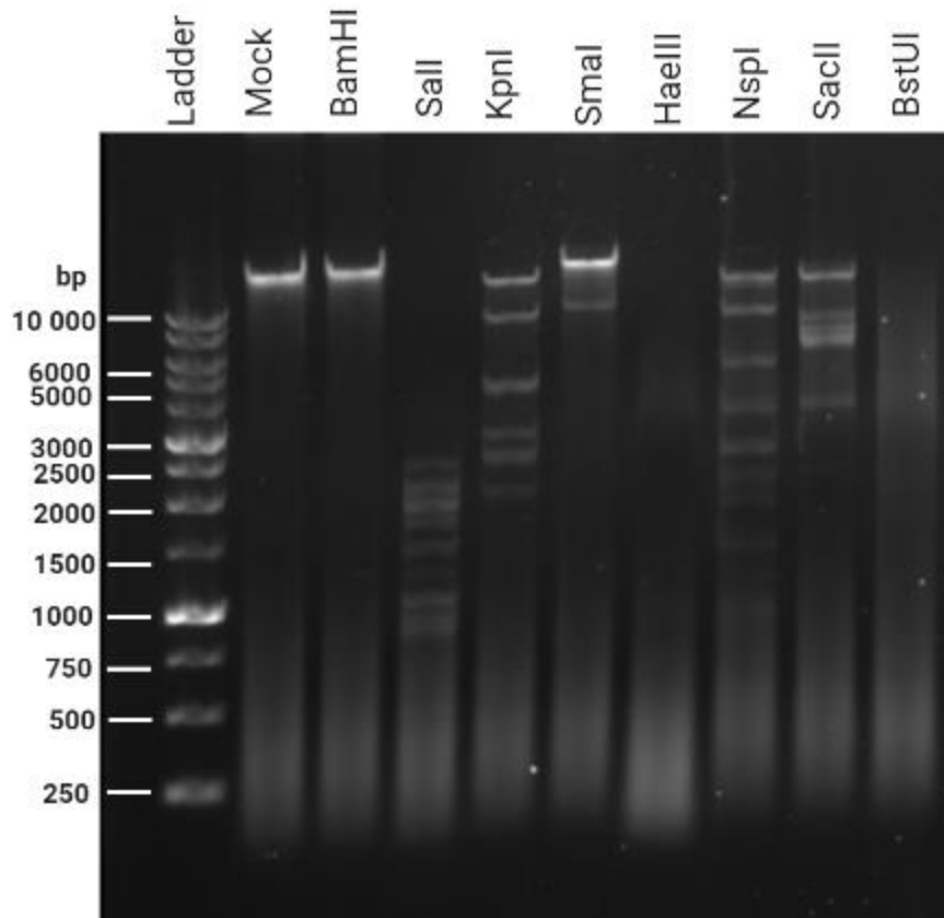
Restriction enzyme digest of the Stevie genome. 500 ng of purified Stevie genomic DNA was digested with the indicated enzymes for 1 hr at 37°C, run on a 1% agarose gel containing 10 µg/ml ethidium bromide, and imaged.
