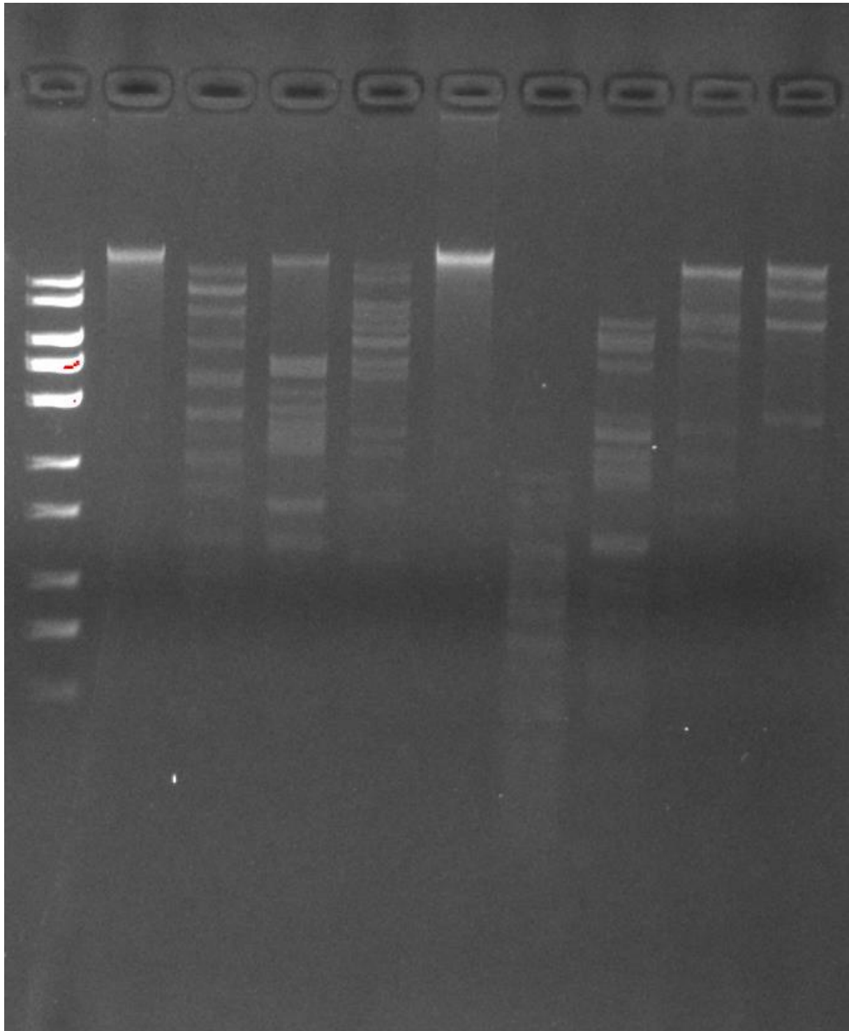
Restriction enzyme digest of Winellie genome. Purified Winellie genomic DNA was digested with the indicated enzymes for 1hr at 37°C, un on a 1% agarose gel containing 10µg/ml ethidium bromide and imaged.
