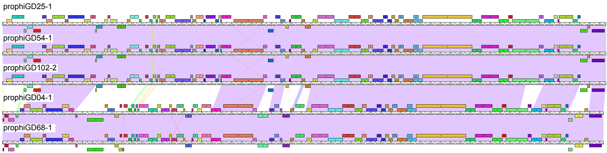
Figure S14. Genome comparisons of ClusterMabE1. See Figure S3 for details.
