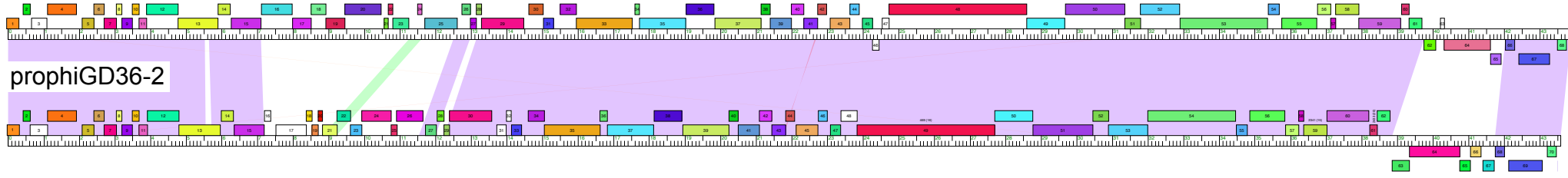
Figure S21. Genome comparison of MabH phages. See Figure S3 for details.
