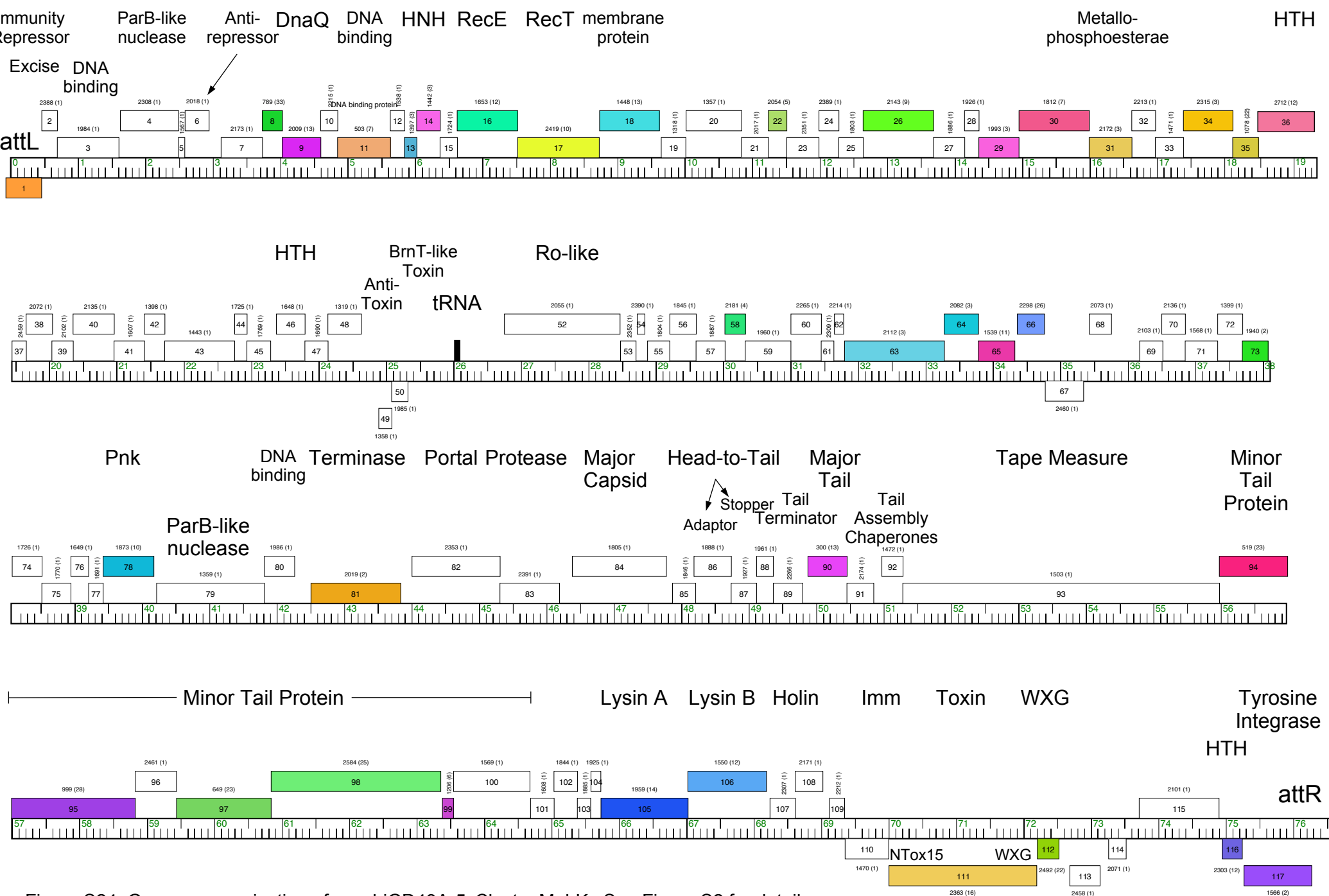
Figure S24. Genome organization of prophage GD43A-5, Cluster MabK. See Figure S2 for details.
