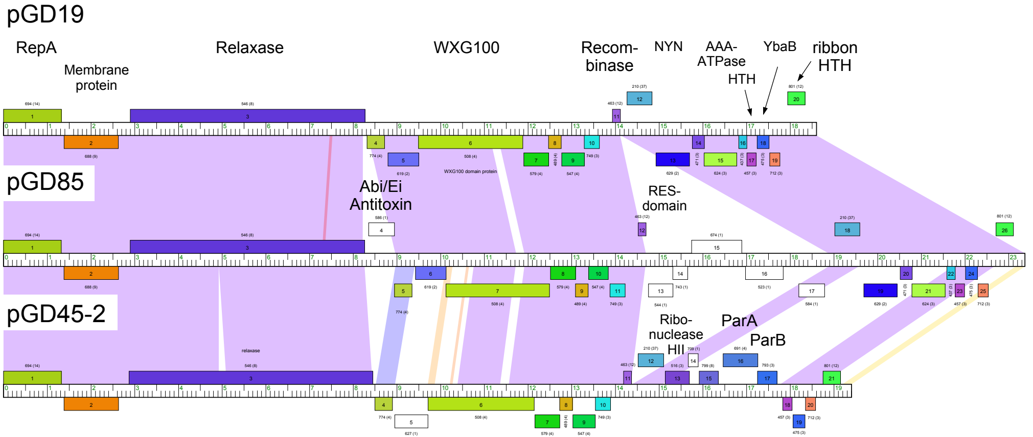
Figure S37. Genome organization and comparisons of Cluster pD. See Figure S33 for details.
