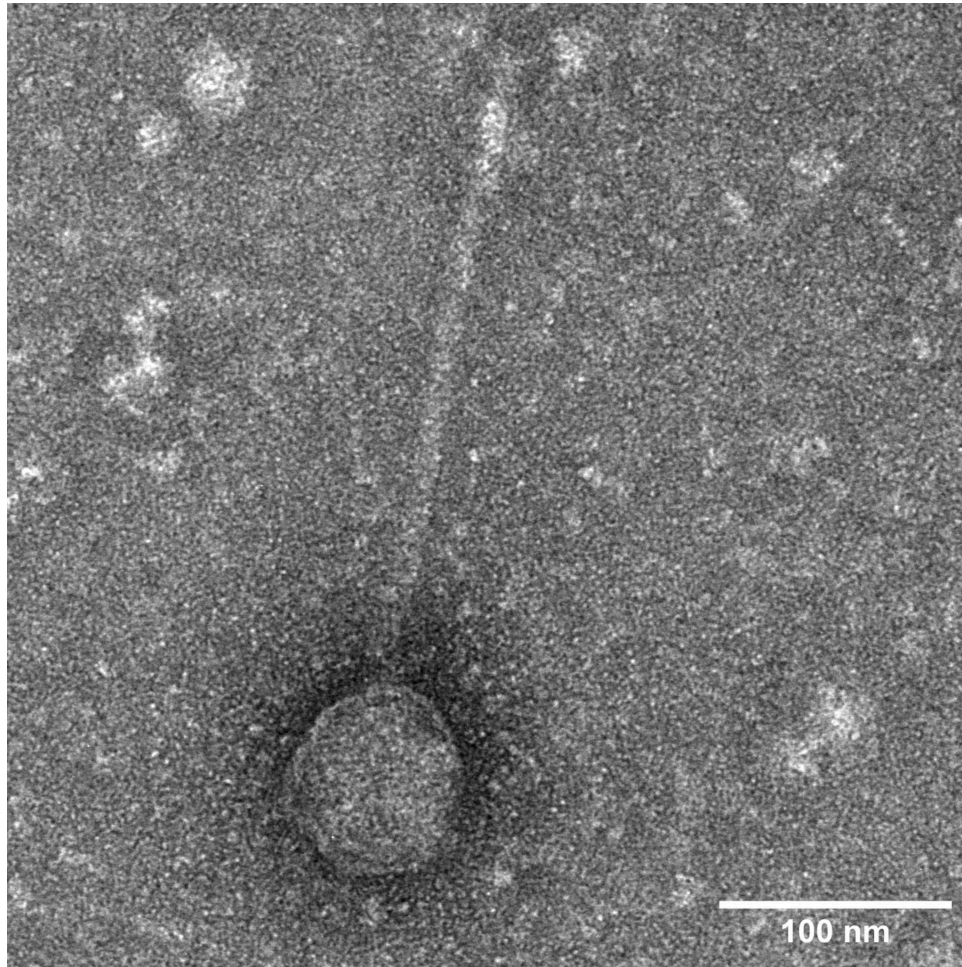
TEM image of bacteriophage Agnodice . 10 \mu l filtered lysate was placed on a TEM grid and treated with 10 \mu l of 1% uranyl acetate as a negative stain. The image was opened and adjusted using Fiji ImageJ software.
