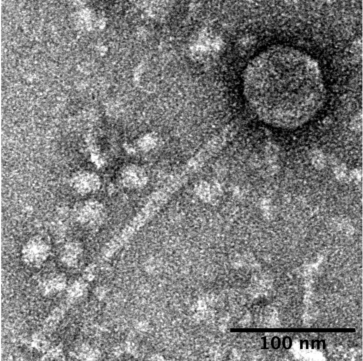
Transmission electron micrograph of Ambassador. Phage was imaged at 120 kV and counter-stained with 1% uranyl acetate. The capsid is 64 nm wide, and the tail is 249 nm long and 12 nm wide.
