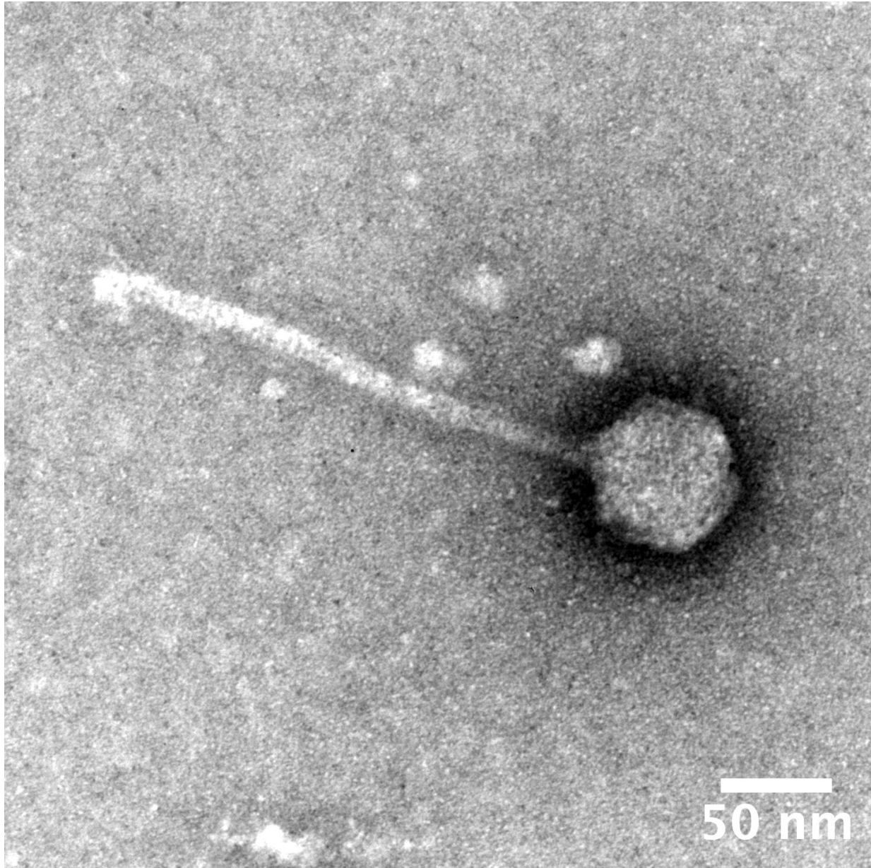
Transmission electron micrograph of Charbel. Charbel was stained with 1% uranyl acetate and imaged at 120 kV. The capsid is 65.60 nm wide, and its tail length is 226.46 nm.
