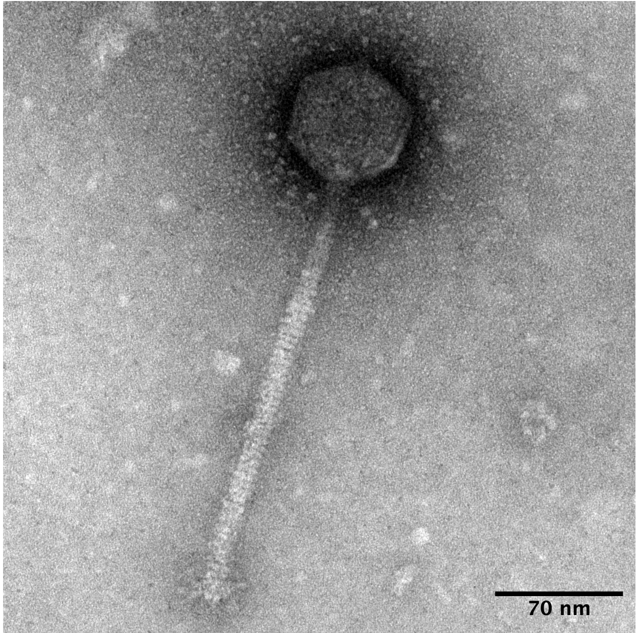
Transmission electron micrograph of Dalian . Dalian was stained with 1% uranyl acetate and imaged at 120 kV. The tail length is on average 227.0649 \pm 3.0398 nm, the tail width is on average 11.1792 \pm 0.4463 nm. The capsid width is on average 61.827 \pm 2.413 nm.
