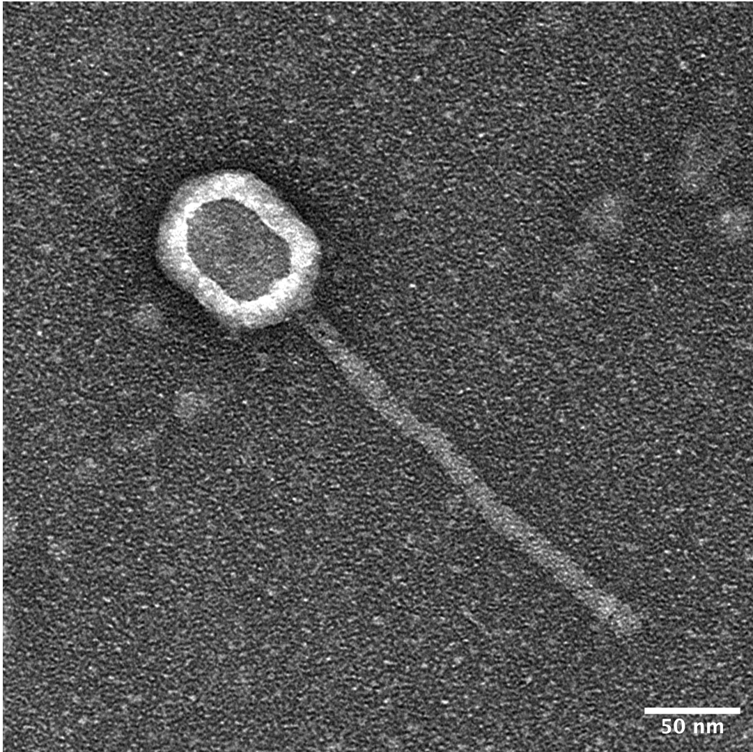
Transmission electron micrograph of DibsRuman . DibsRuman was stained with 1% uranyl acid and imaged at 120kV. The capsid is 67.8nm long, and it's tail length is 242.0nm.
