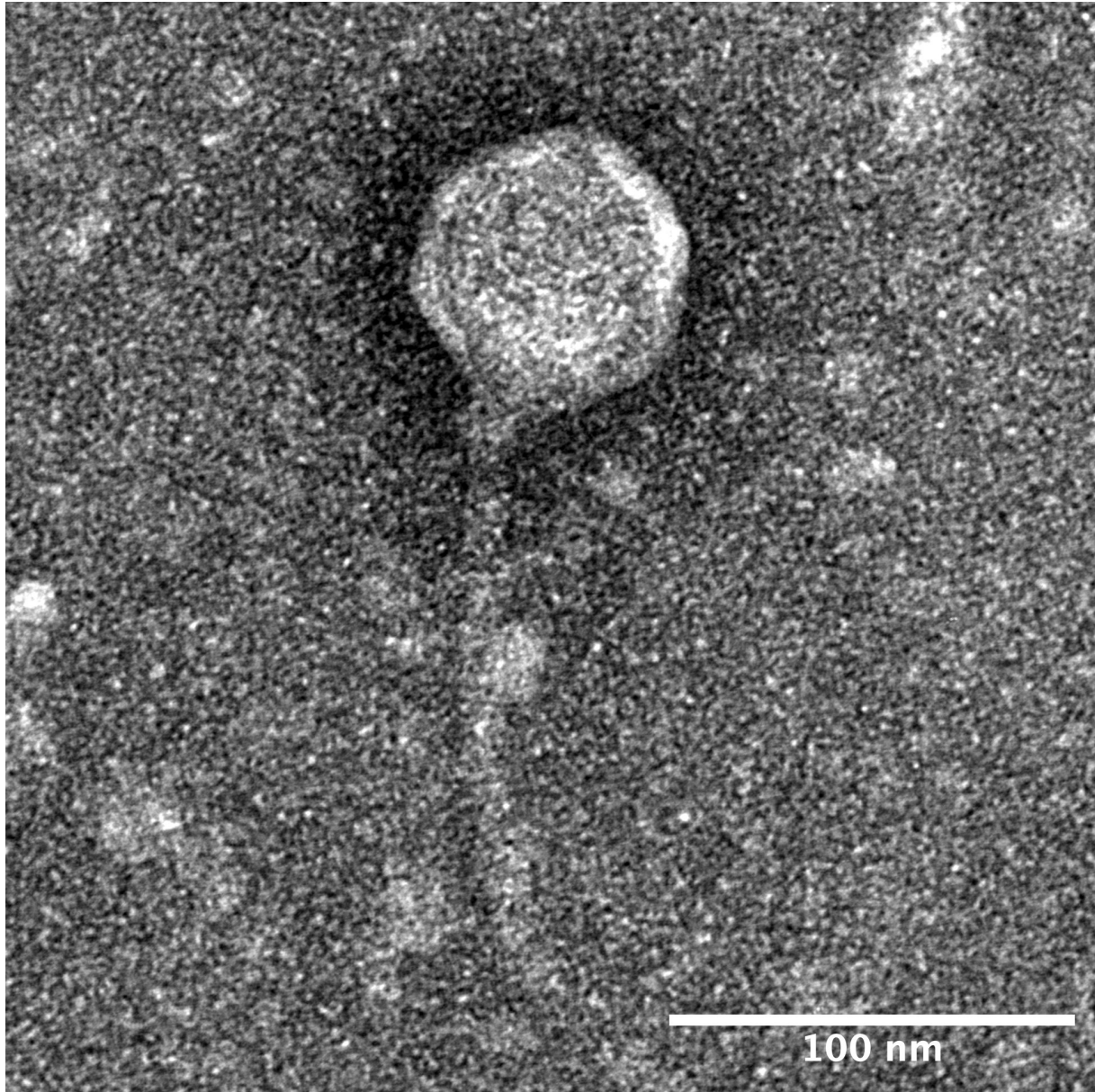
Transmission Electron Microscopy (TEM) Image of the Bacteriophage, Ewoo. Ewoo stained with 1% uranyl acetate and imaged. Scale bar represents 100nm. Capsid width of Ewoo is 64.46 nm. Tail length is 145.95 nm, and the tail width is 8.96 nm.
