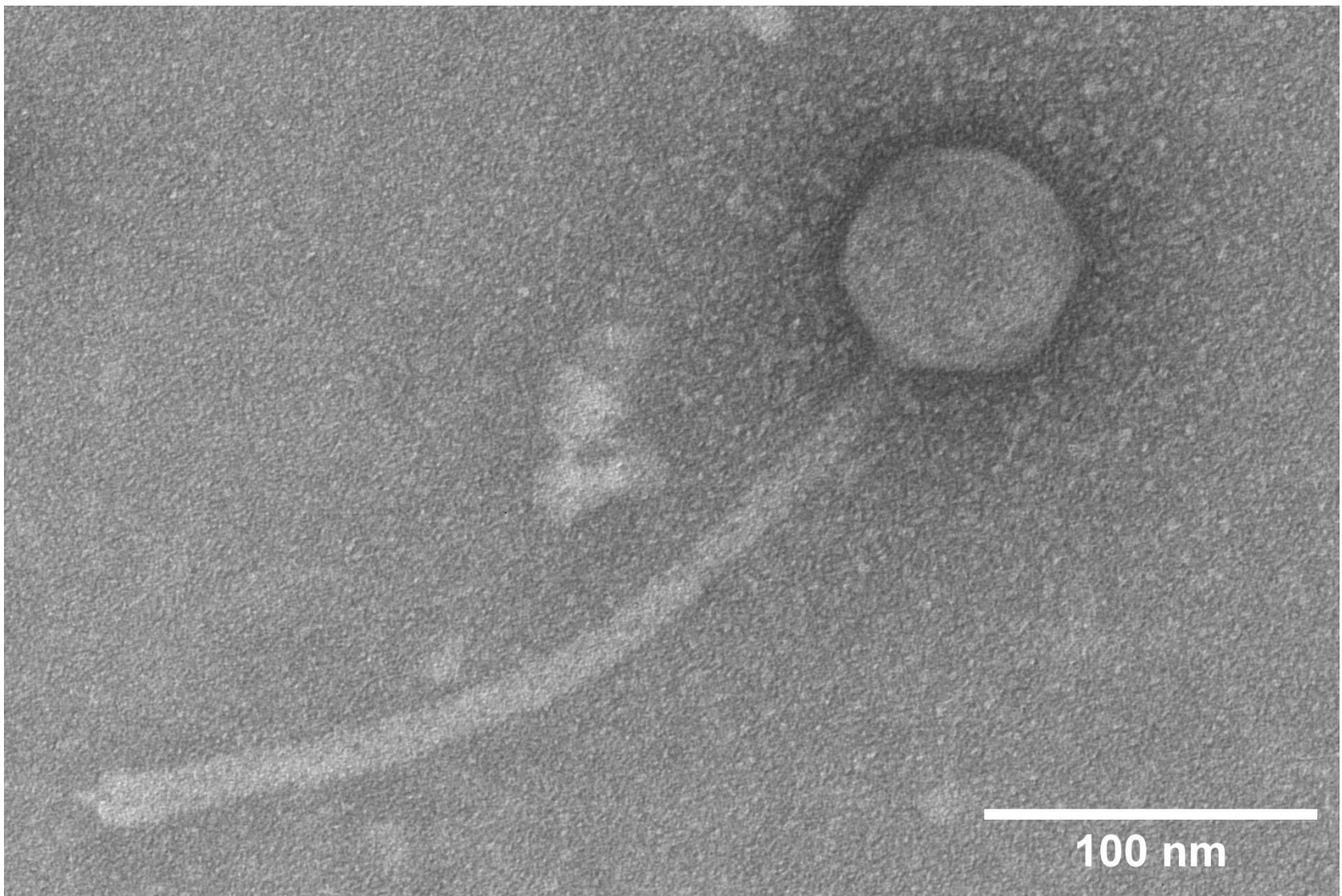
Transmission electron micrograph of Fergusina. Fergusina was stained with 1% uranyl acetate and imaged at 110 kV. The capsid is 68.9 \text{ nm} \pm 0.5 wide, and its tail length is 271.4 \pm 0.1 \text{ nm} .
