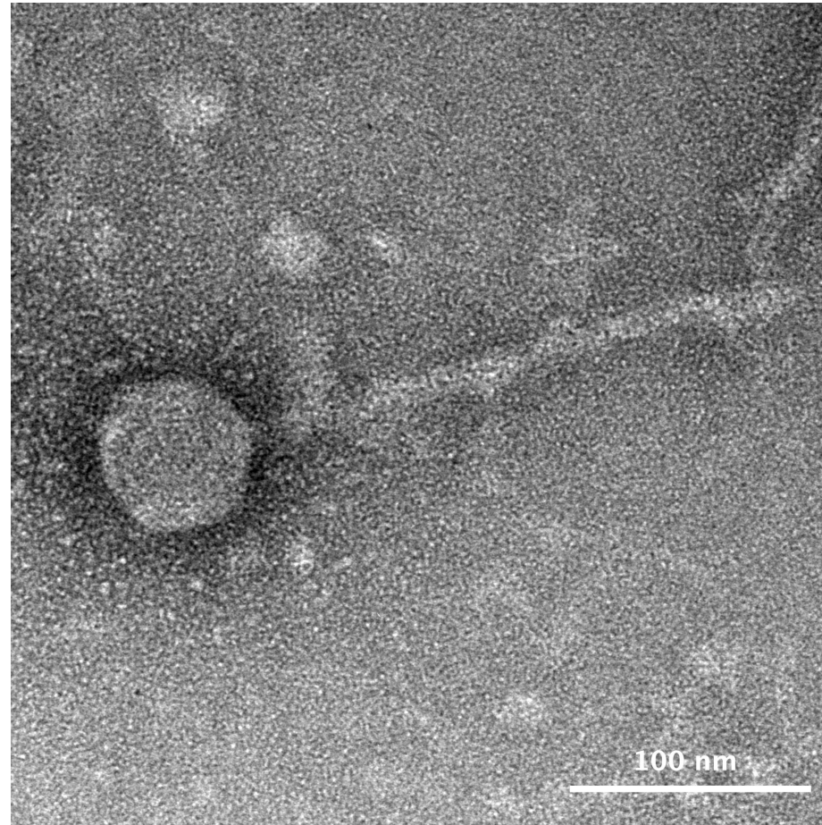
Transmission electron micrograph of Invermay. Invermay was stained with 1% uranyl acetate and imaged at 120 kV. The capsid is 66 nm wide and 63 nm long, and its tail length is 234 nm.
