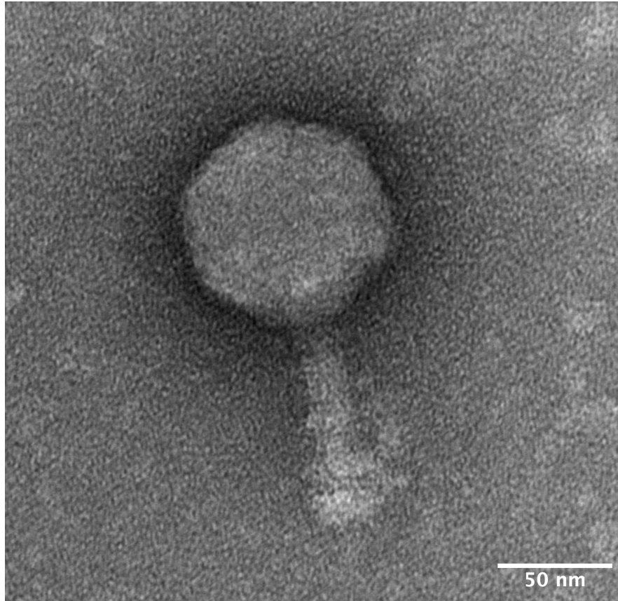
Transmission electron micrograph of Jask. Jask was stained with 1% uranyl acetate and imaged at 120 kV. The capsid is 90.893 nm wide, and its tail is 85.257 nm long and 17.468 nm wide.
