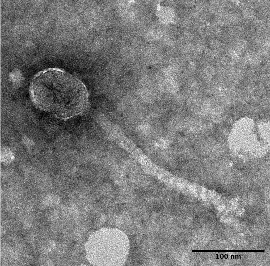
Transmission electron micrograph of JeffKlug. JeffKlug was stained with 1% uranyl acetate and imaged at 120 kV. The prolate capsid is 61 nm wide and 83 nm long, and its tail length is 243 nm.
