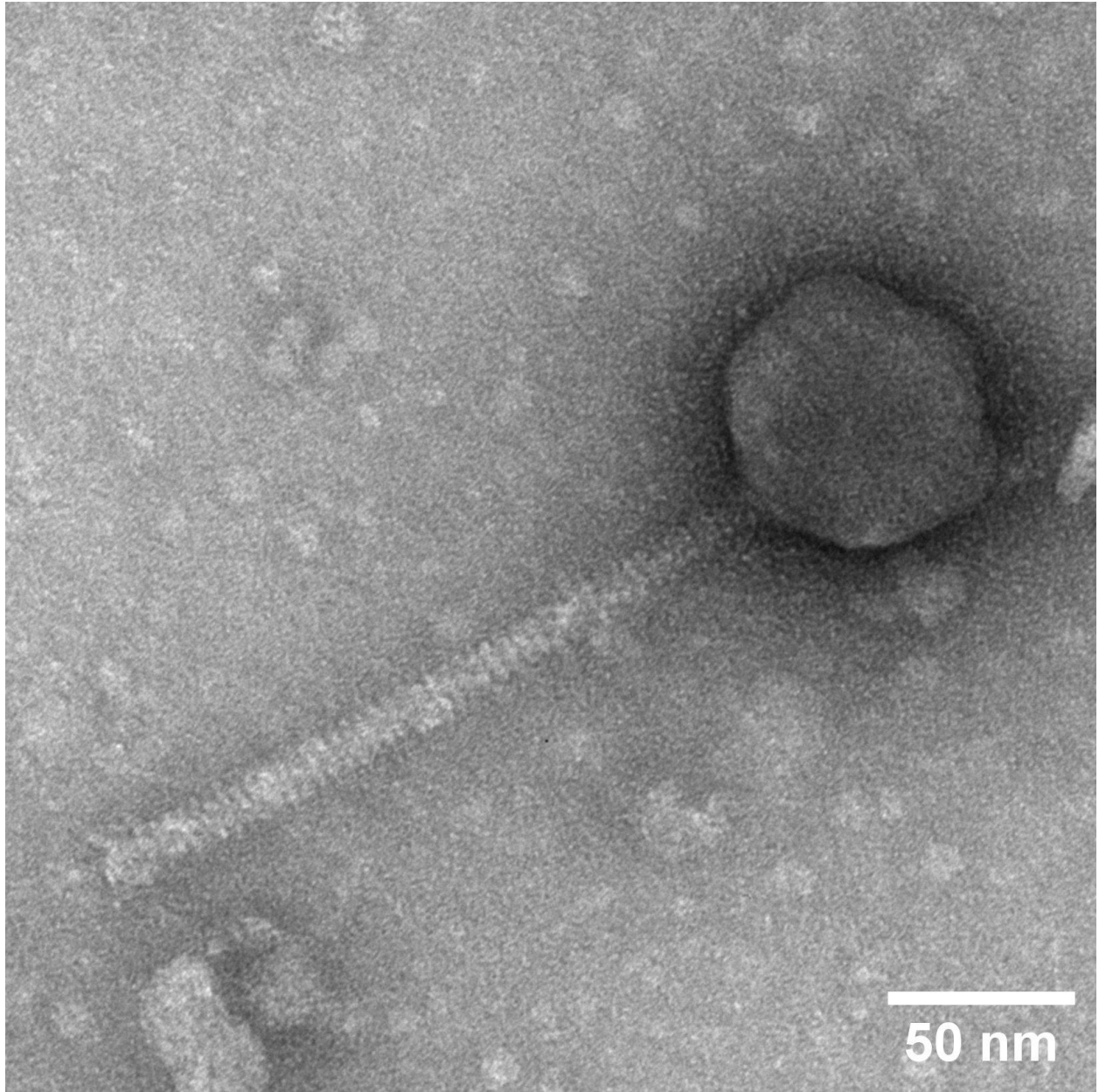
Transmission electron micrograph of Joumoune. Joumoune was stained with 1% uranyl acetate and imaged at 120kV. The capsid width is 75.25 nm, and height is 69.14 nm. The tail width is 13.42 nm, and the length is 199.38 nm.
