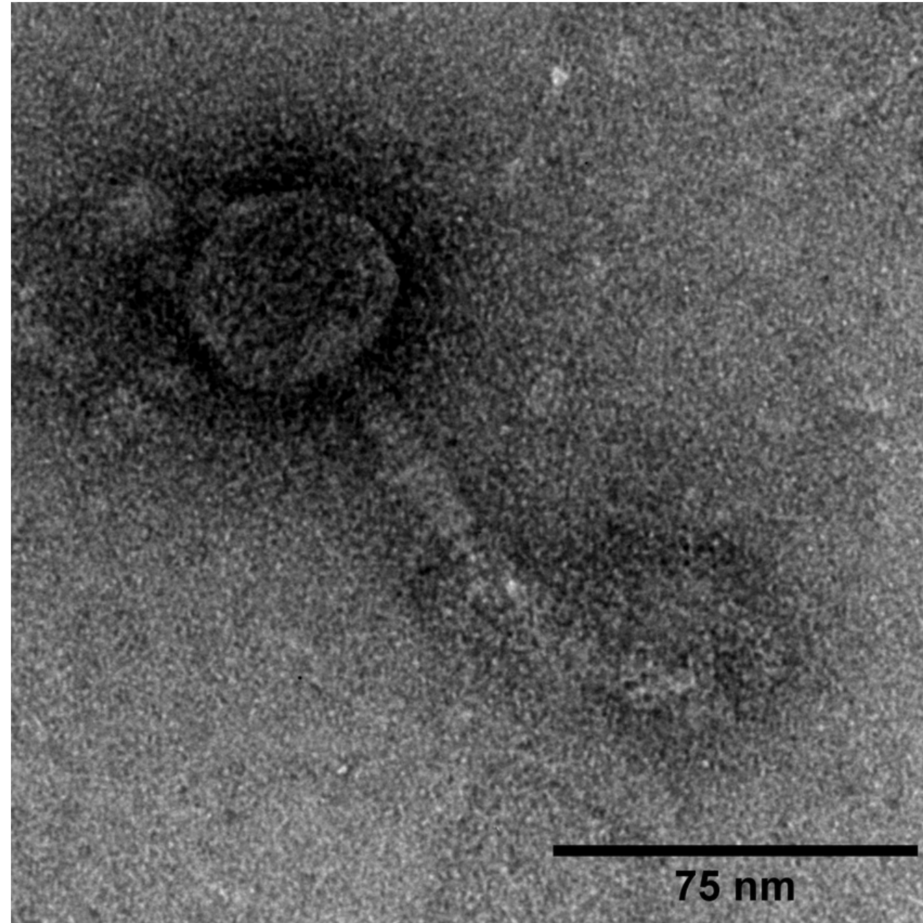
Transmission electron micrograph of Liebestraum. Liebestraum was negatively stained with 1% uranyl acetate and imaged at 120kV. The tail length is 112nm and the capsid width is 43nm.
