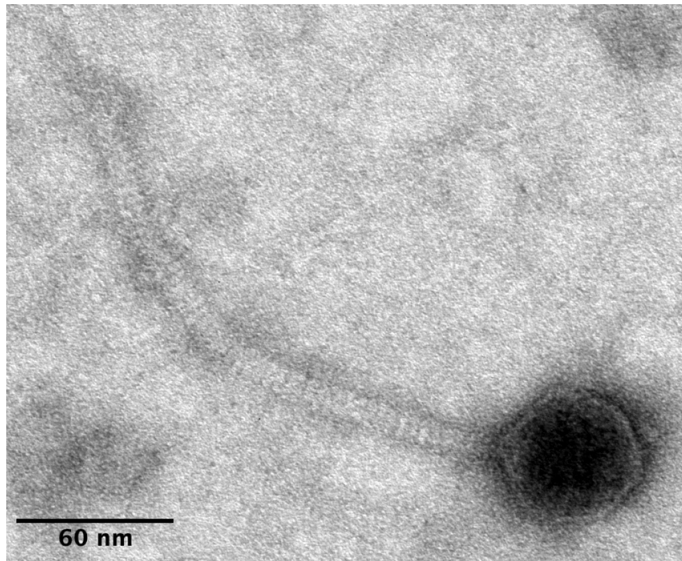
Transmission Electron Micrograph of Martlet Bacteriophage. Martlet was stained with 1% uranyl acetate and imaged at 120 kV. The capsid has an average measured width of 45.9 nm. The tail has an average measured length of 209.9 nm.
