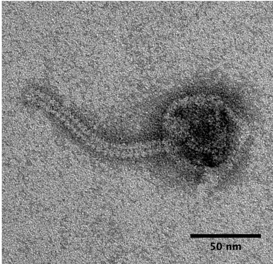
Transmission electron micrograph of Maynay . Negative staining technique with 1% uranyl acetate was used to image Maynay at 120 kV. The capsid is 52.3 \text{ nm} \pm 1.42 wide and the tail is 119.5 \text{ nm} \pm 0.63 long.
