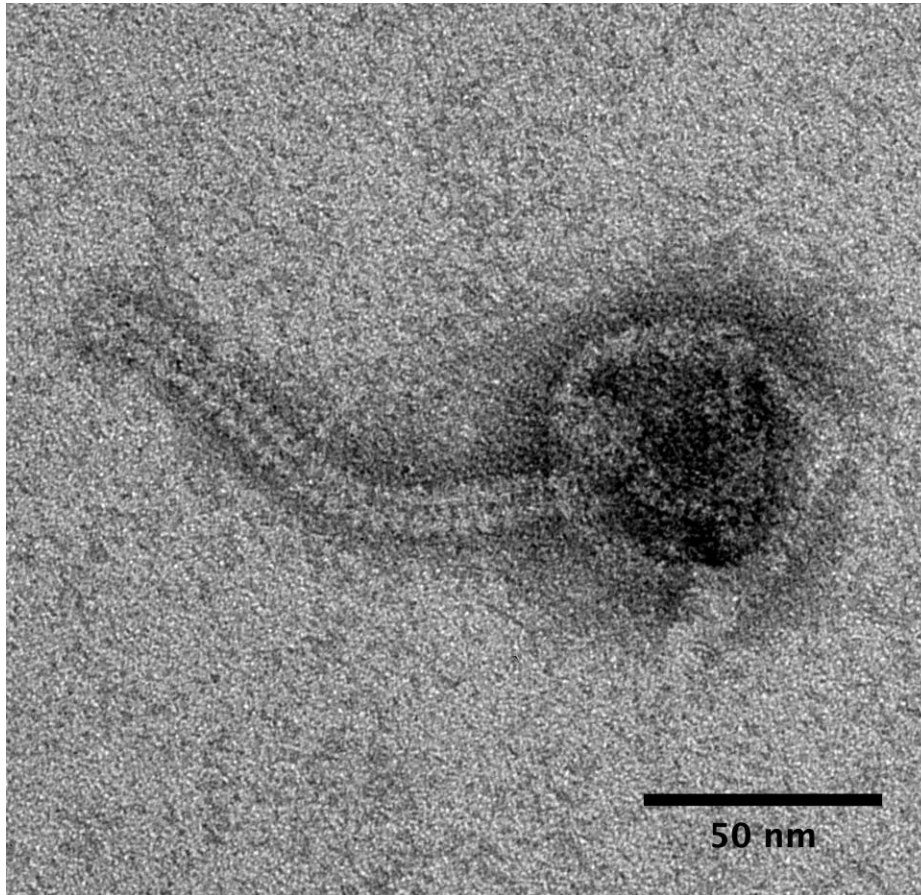
Transmission electron micrograph of Maynay . Negative staining technique with 1% uranyl acetate was used to image Maynay at 120 kV. The capsid is 52.3 \text{ nm} \pm 1.42 wide and 53.5 \text{ nm} \pm 3.76 long. The tail is 119.5 \text{ nm} \pm 0.63 long.
