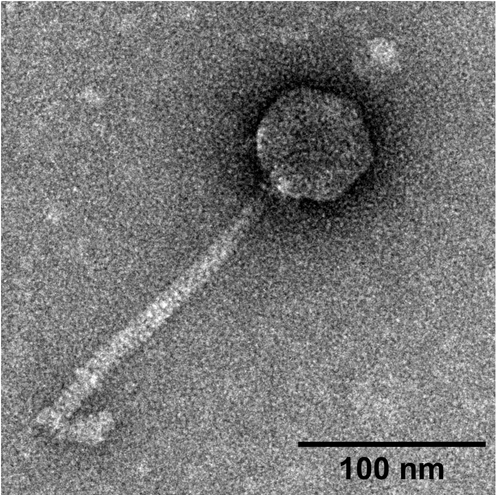
Transmission electron micrograph of MimiCo. MimiCo was stained with 1% uranyl acetate and imaged at 120 kV.
