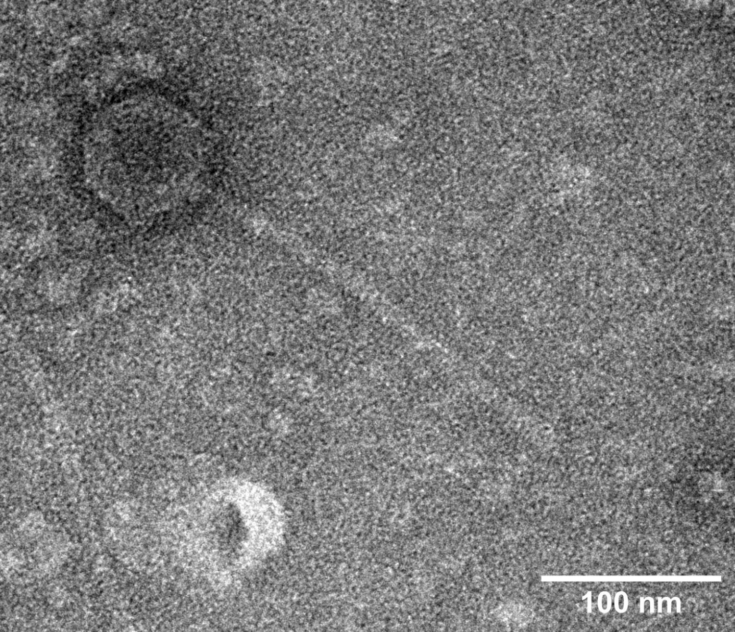
Transmission electron micrograph of Onionphile. The TEM grid containing Onionphile was stained with 1% uranyl acetate (UA) prior to imaging at 120 kV. The capsid measures 63 nm in width, while the tail has a length of 233 nm.
