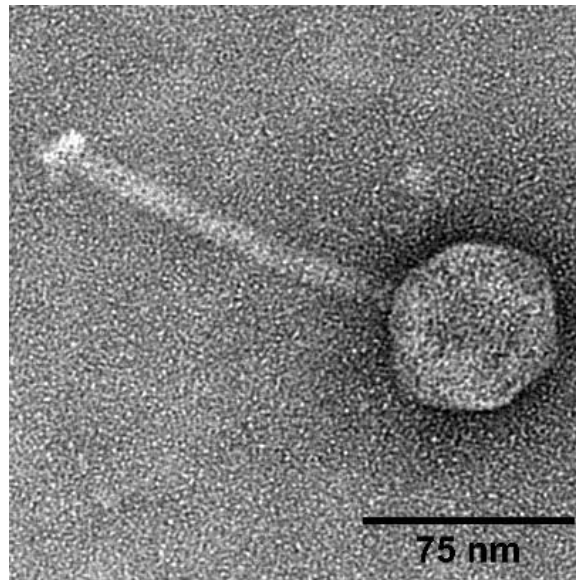
Transmission electron micrograph of Phrass . Phrass was stained with 1% uranyl acetate. The tail length is approximately 129.5 nm while the capsid length is approximately 59.9nm
