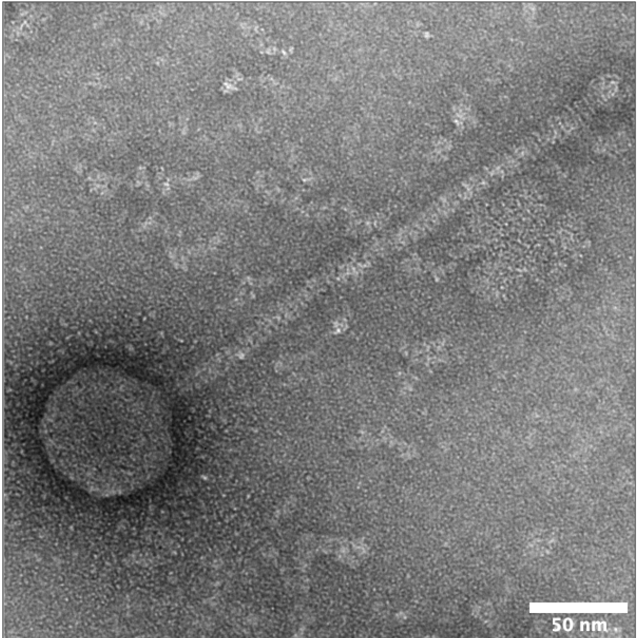
TEM image of phage Pollock. Type-B, 300 mesh, Formvar Copper coated grid was soaked with high titer lysate and negatively stained with 1% uranyl acetate. Grids were dried and imaged at 120kV using transmission electron microscopy. Average tail length of 269.84 nm and capsid diameter of 67.16 nm obtained from three images.
