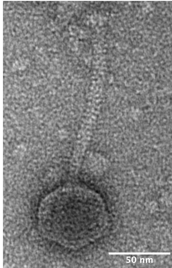
Transmission Electron Microscopy (TEM) image of Scoobydoodoo . Scoobydoodoo was stained with 1% UA and then imaged with a TEM at 120kV. The capsid width and tail length are 56.6nm and 116.5nm respectively and these measurements were obtained with Fiji.
