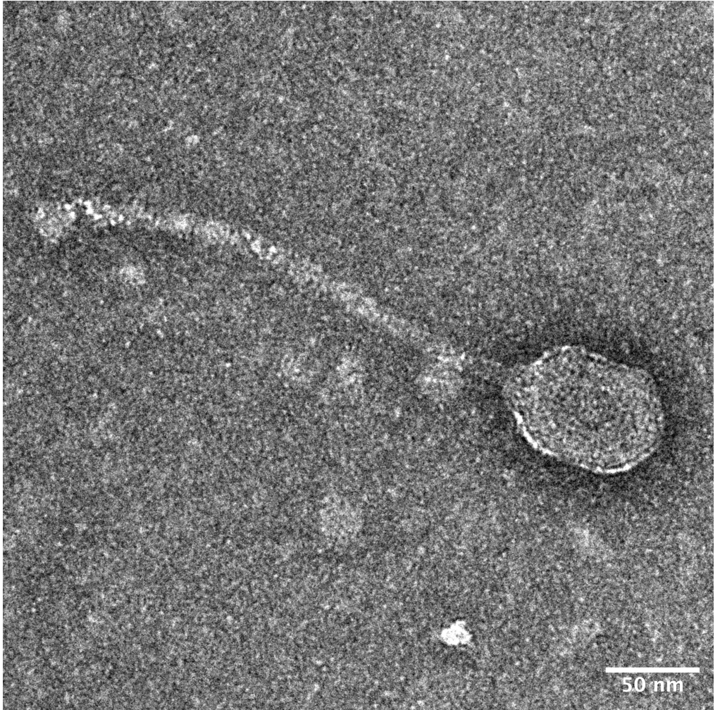
Transmission electron micrograph of Soytoy. Soytoy was stained with 1% uranyl acetate and imaged at 120 kV. The prolate capsid is 58 nm wide and 83 nm long, and its tail length is 273 nm.
