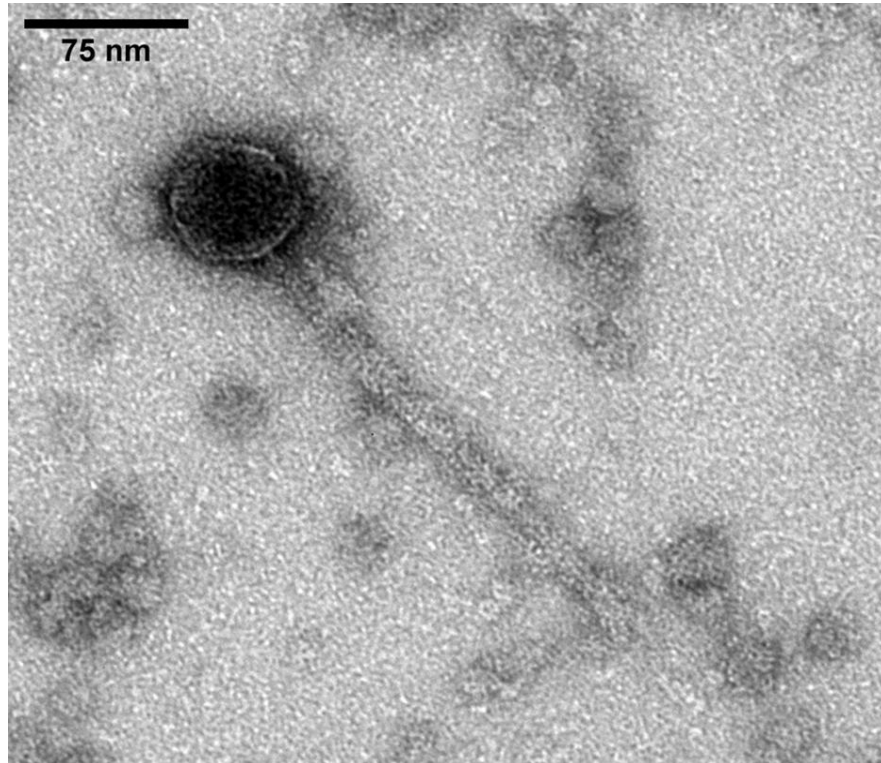
Transmission electron micrograph of the Strava bacteriophage. Phage particles were negatively stained with 1% uranyl acetate and imaged at 120 kV. Morphometric measurements performed in Fiji show an average capsid diameter of 57.76 nm, a tail length of 217.10 nm, and a tail width of 13.93 nm.
