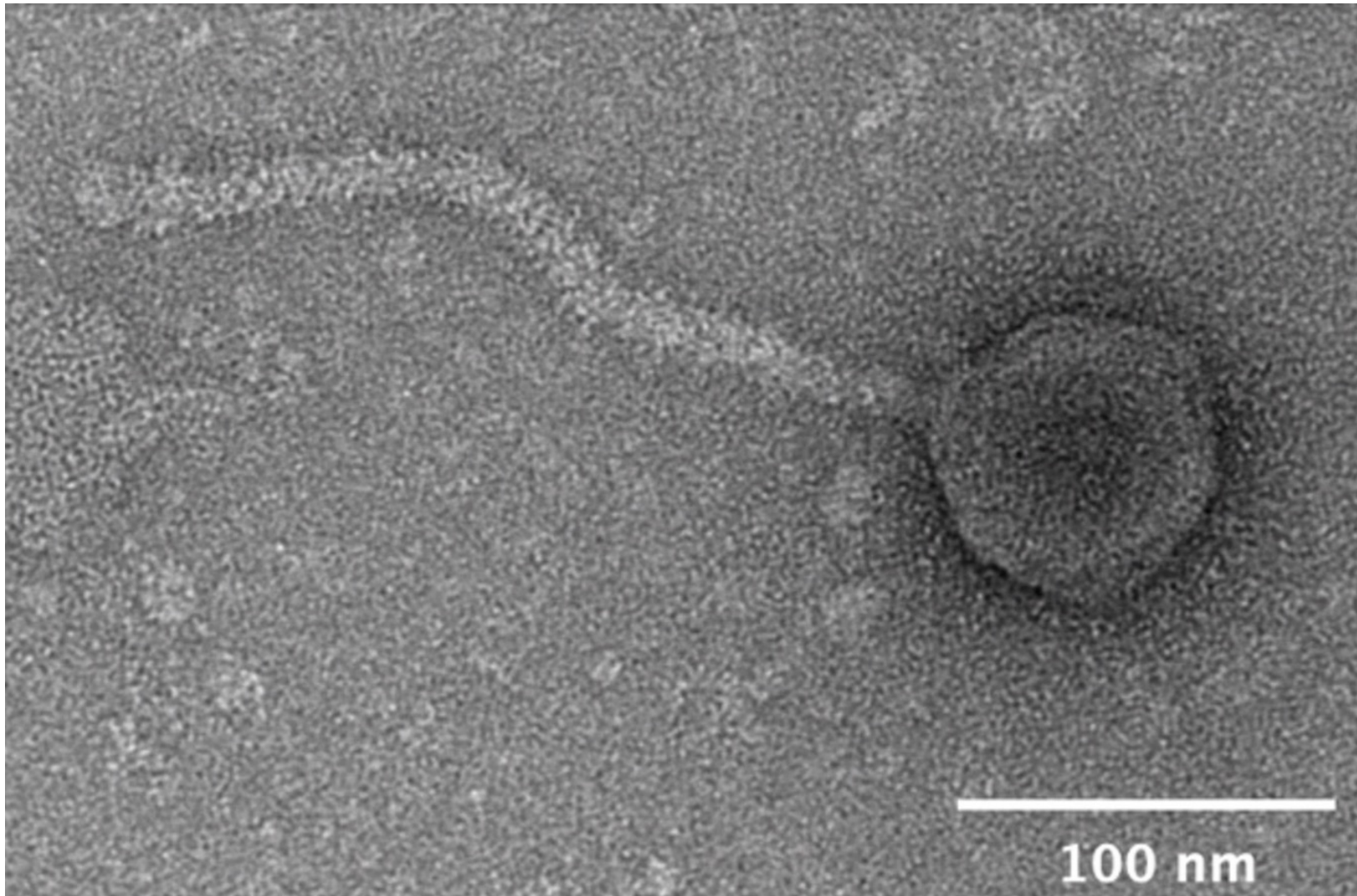
Fig. 2. Transmission electron microscopy (TEM) image of phage Tinish stained with 1% uranyl acetate. Imaging was done at 120 kV. Average capsid width = 74 \pm 0.75 nm. Average tail length = 226 \pm 5.3 nm. n = 9 .
