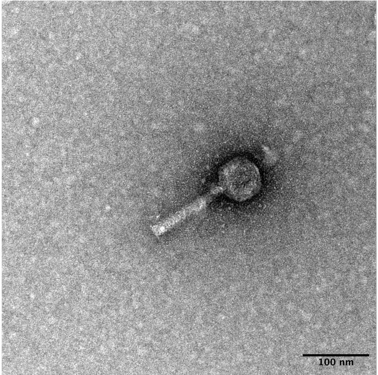
TEM image of bacteriophage Vitus . TEM was performed with 10 \mu L of lysate using a copper grid and 1% uranyl acetate stain.
