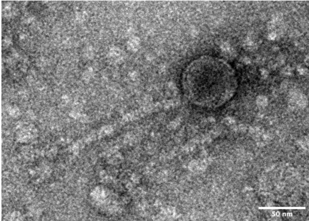
Transmission electron micrograph of Zeita. The TEM grid and Zeita were stained with 1% uranyl acetate (UA) prior to imaging at 120 kV. The capsid measures 55.68 nm in width, while the tail has a length of 128.05 nm.
