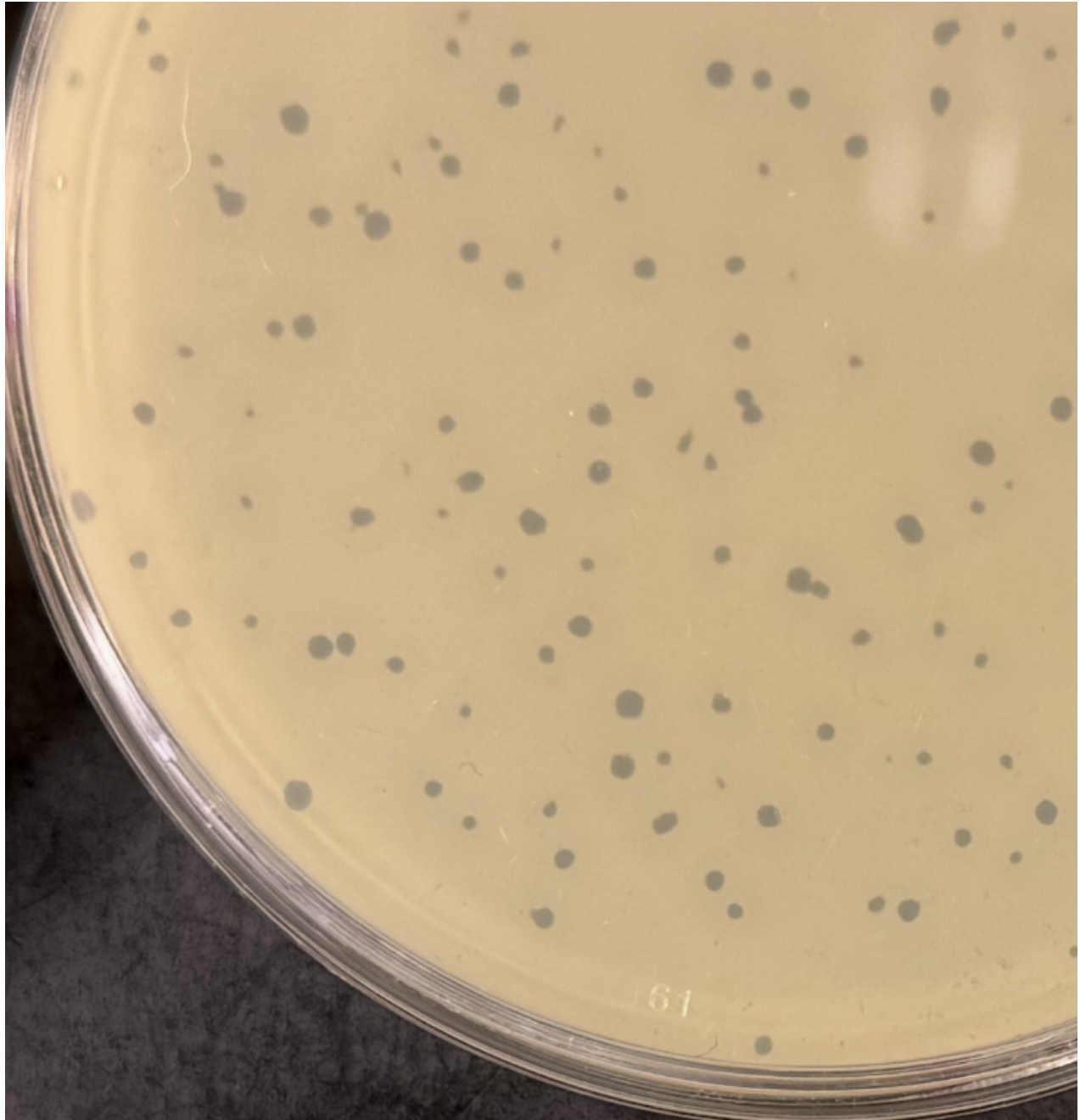
Plaques of Amoria. Approximately 100 bacteriophages were used to infect a culture of Microbacterium foliorum NRRL B-24224. The infected culture was plated using PYCa top agar over a PY agar plate. The plate was then incubated at 30 °C for two days before being imaged
