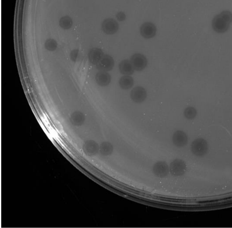
Plaques of Sesshomaru. Around 32 bacteriophages were used to infect a culture of A. globiformis and plated with top agar on a PYCa plate. The plate was incubated for 36 hrs at 30°C and imaged with the Bio-Rad imager.
